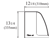
TOMD-L : Side View
