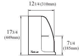
TOMD-H : Side View
